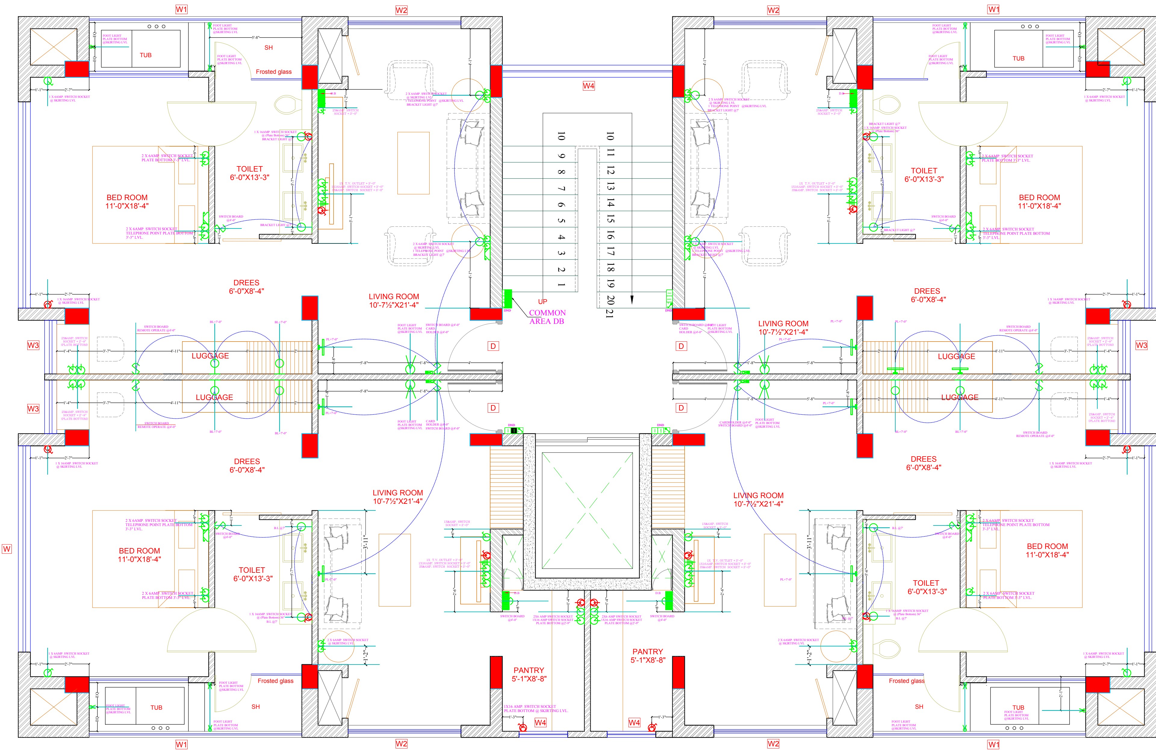
TYPICAL FLOOR WALL ELECTRICAL PLAN
