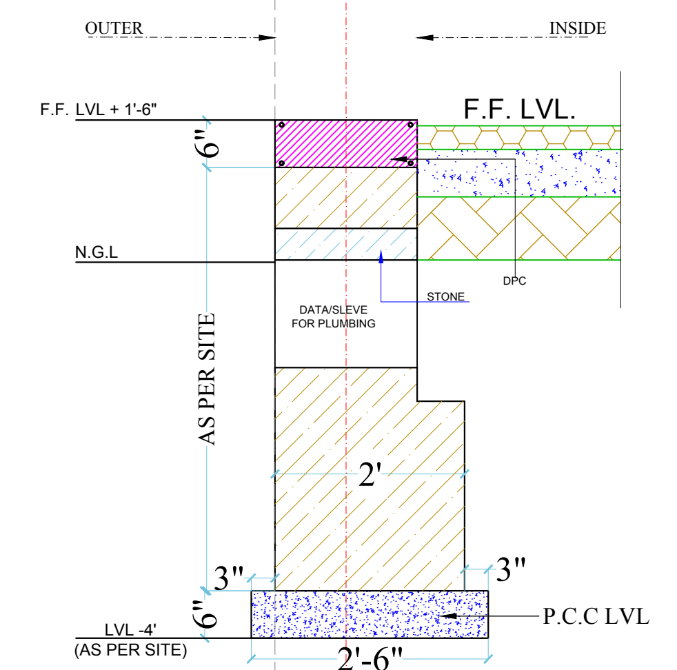
SECTION THRU SLEEVE/DATA
