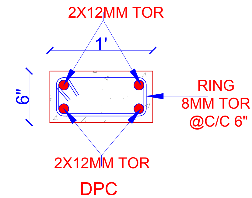
SECTION X1
