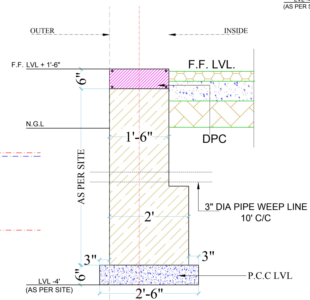
SECTION X2
