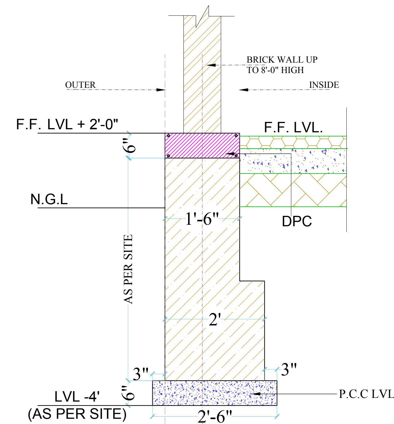
SECTION X1
