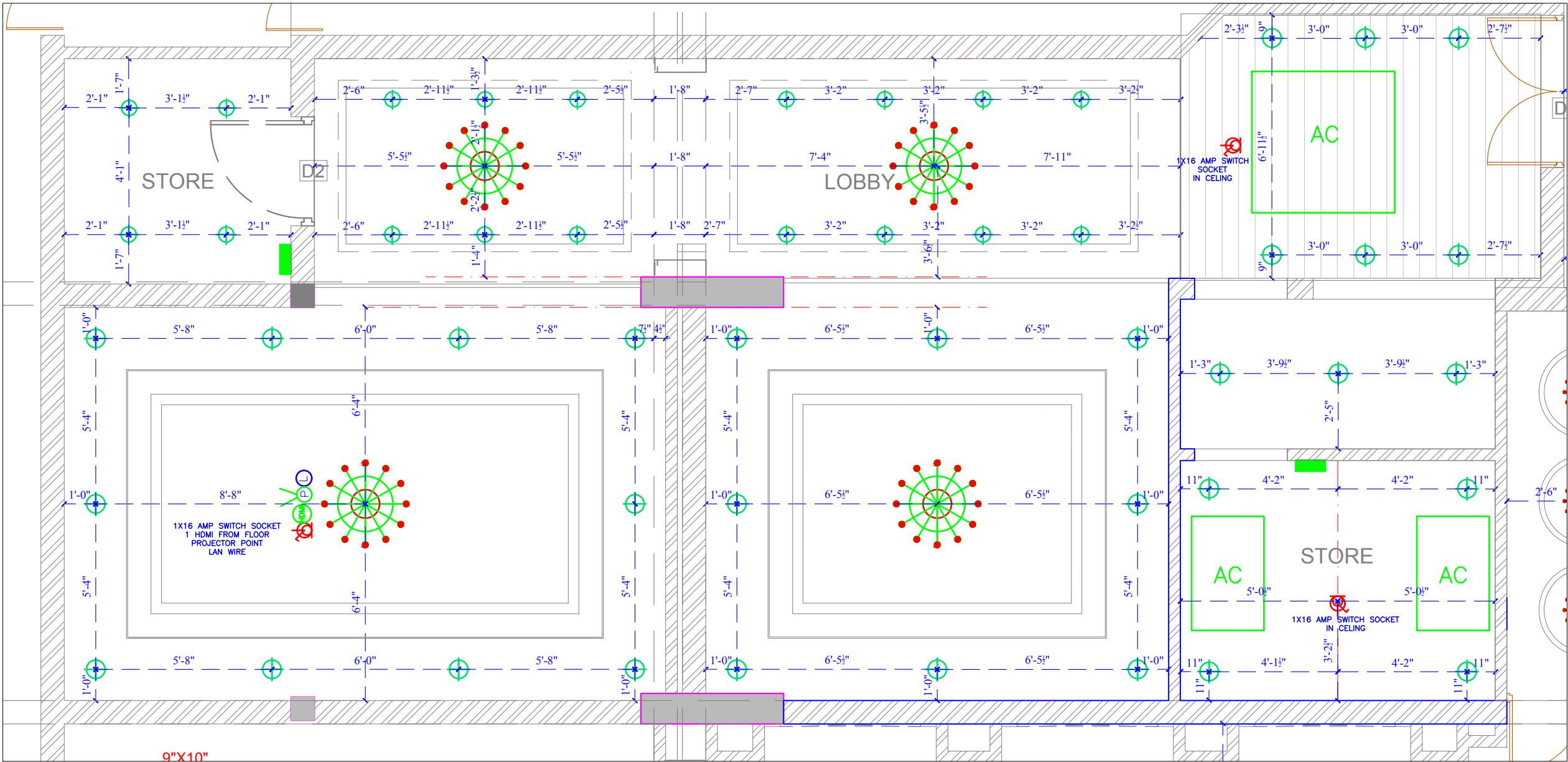
BUSINESS CENTER REFLECTED CEILING ELECTRICAL
