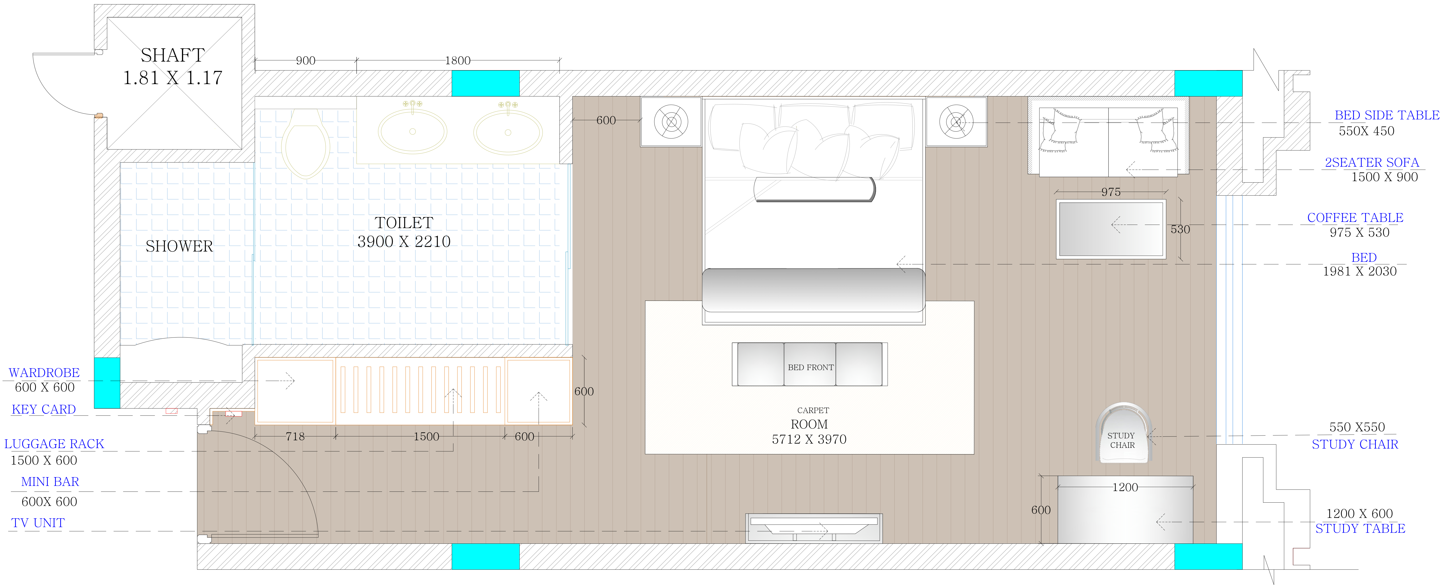
LAYOUT OPT 3
