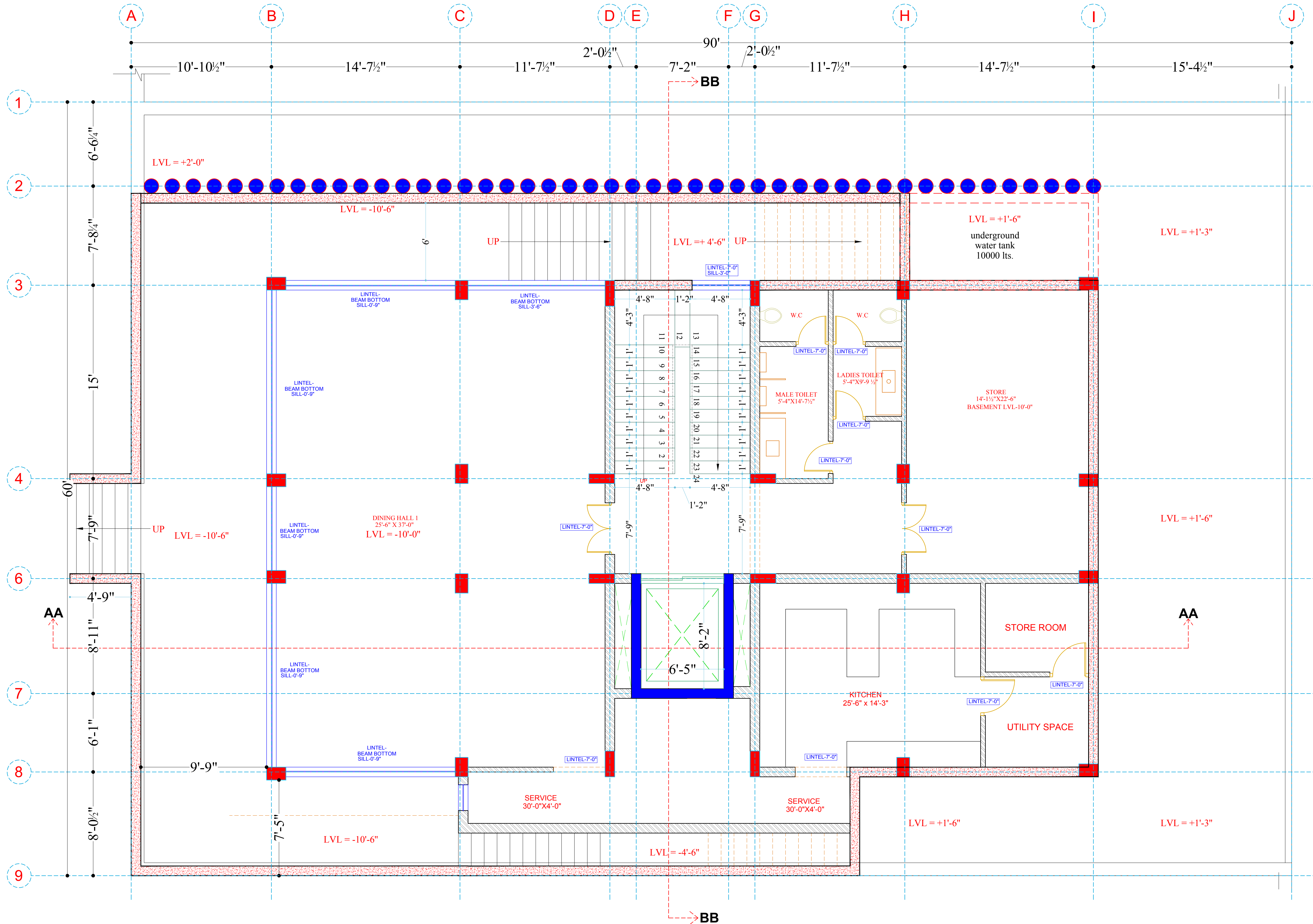
BASEMENT FLOOR
