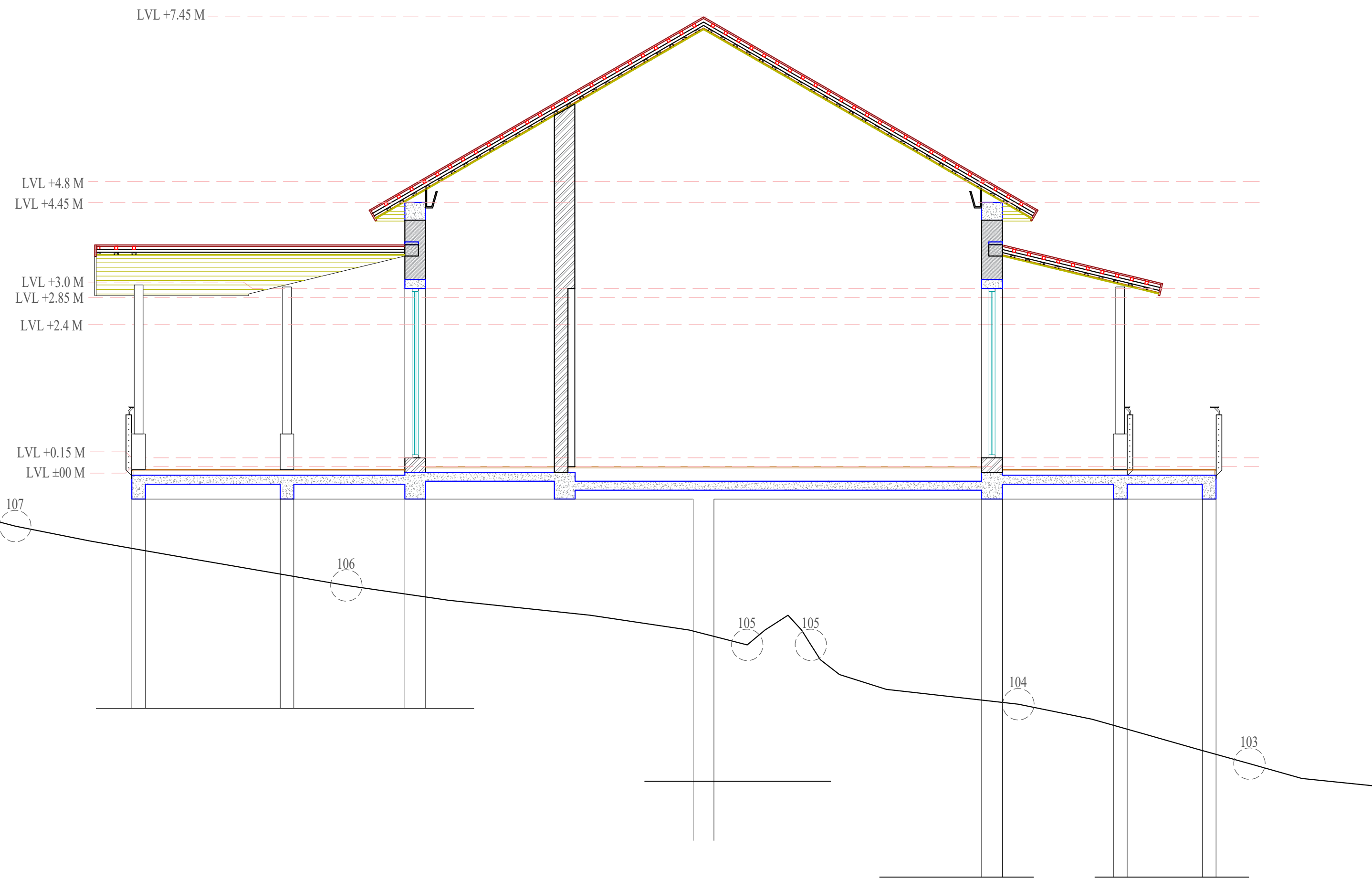
Section CC
