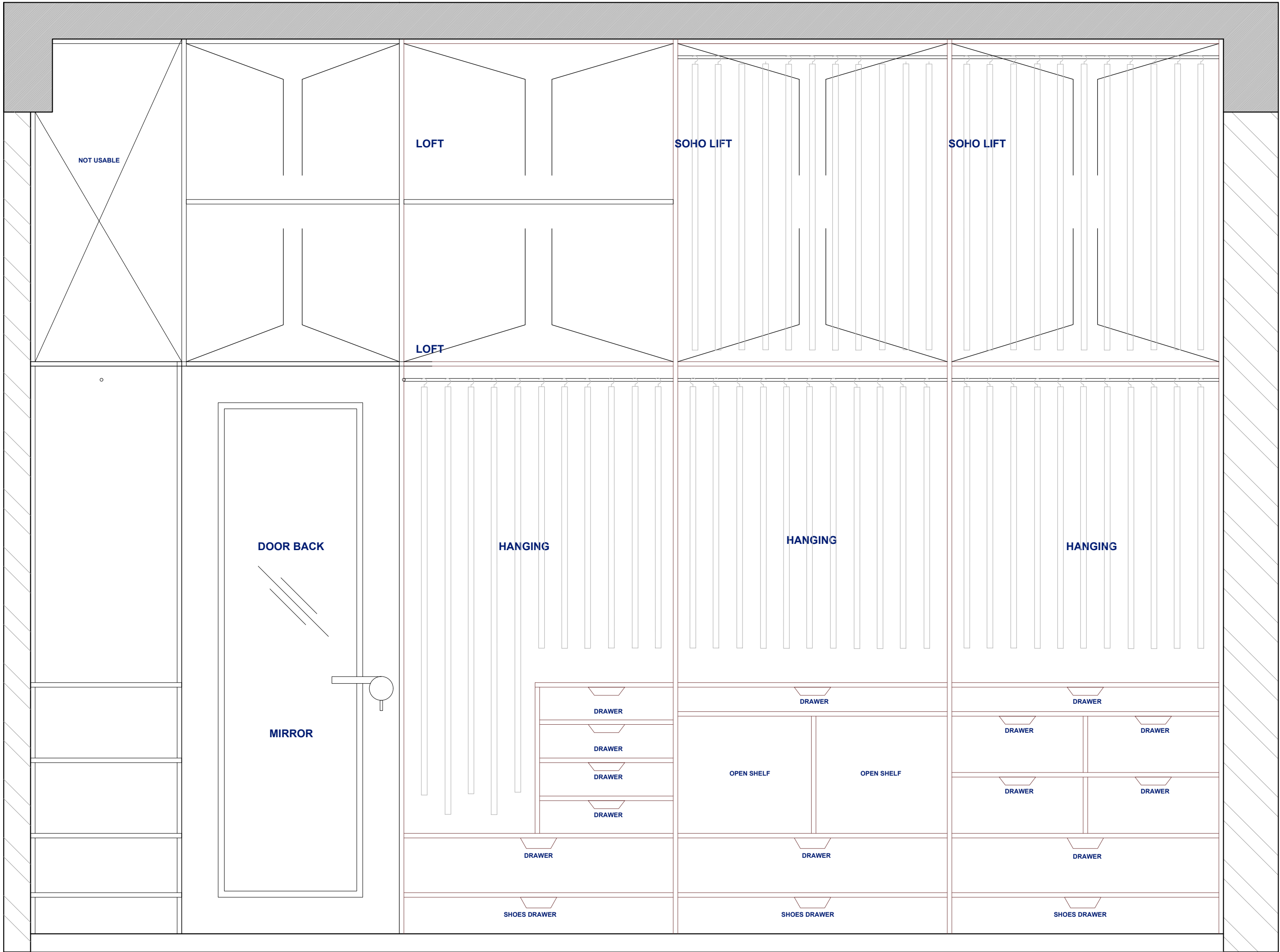
WARDROBE ELEVATION B
