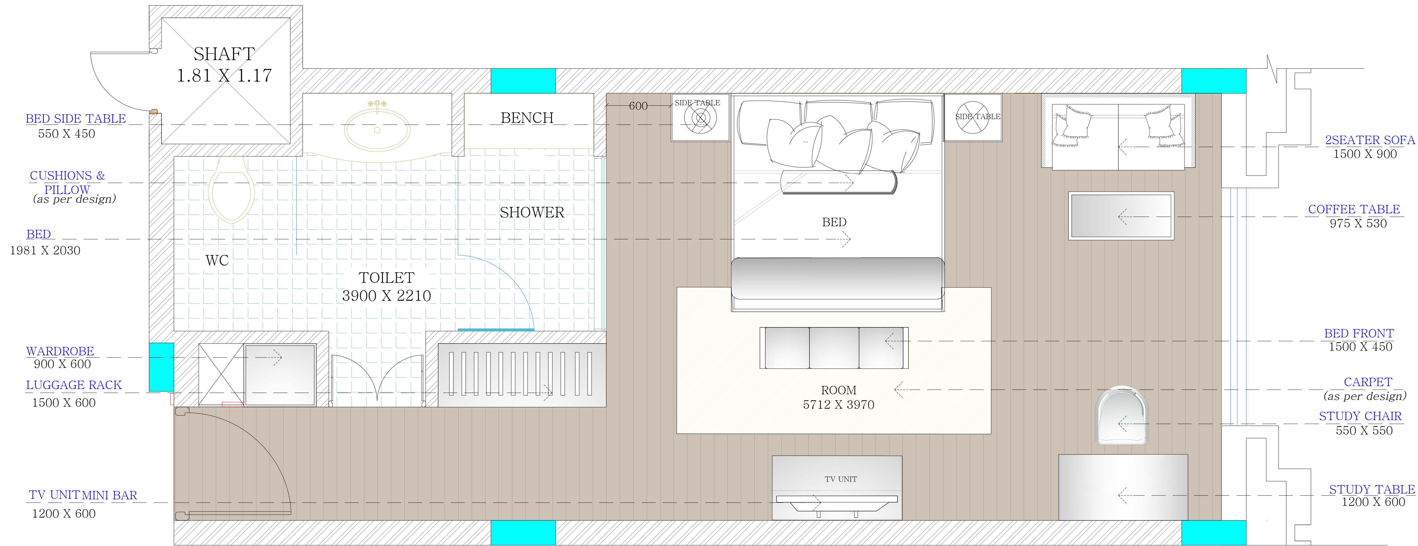
LAYOUT OPT 2
