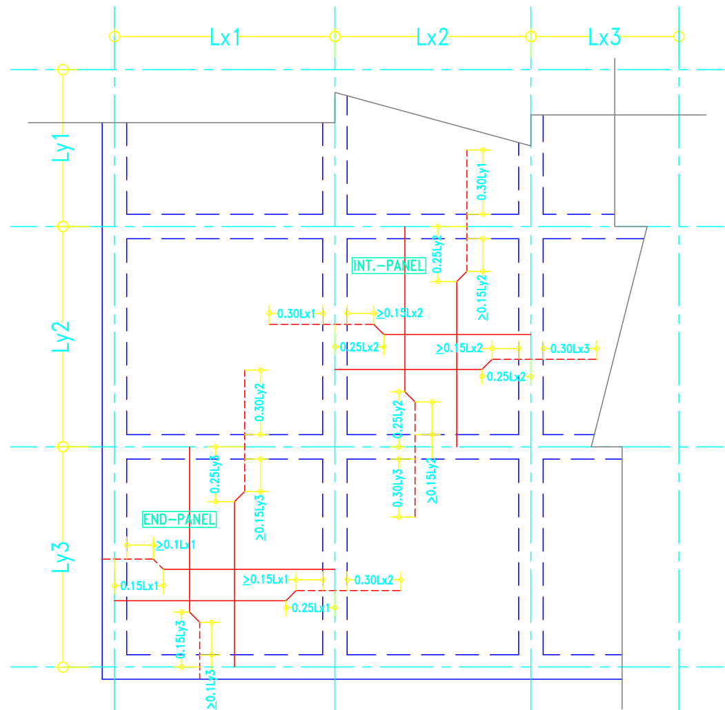
TYPICAL ARRANGEMENTS OF SLAB REINFORCEMENT USING BENT-UP BARS
