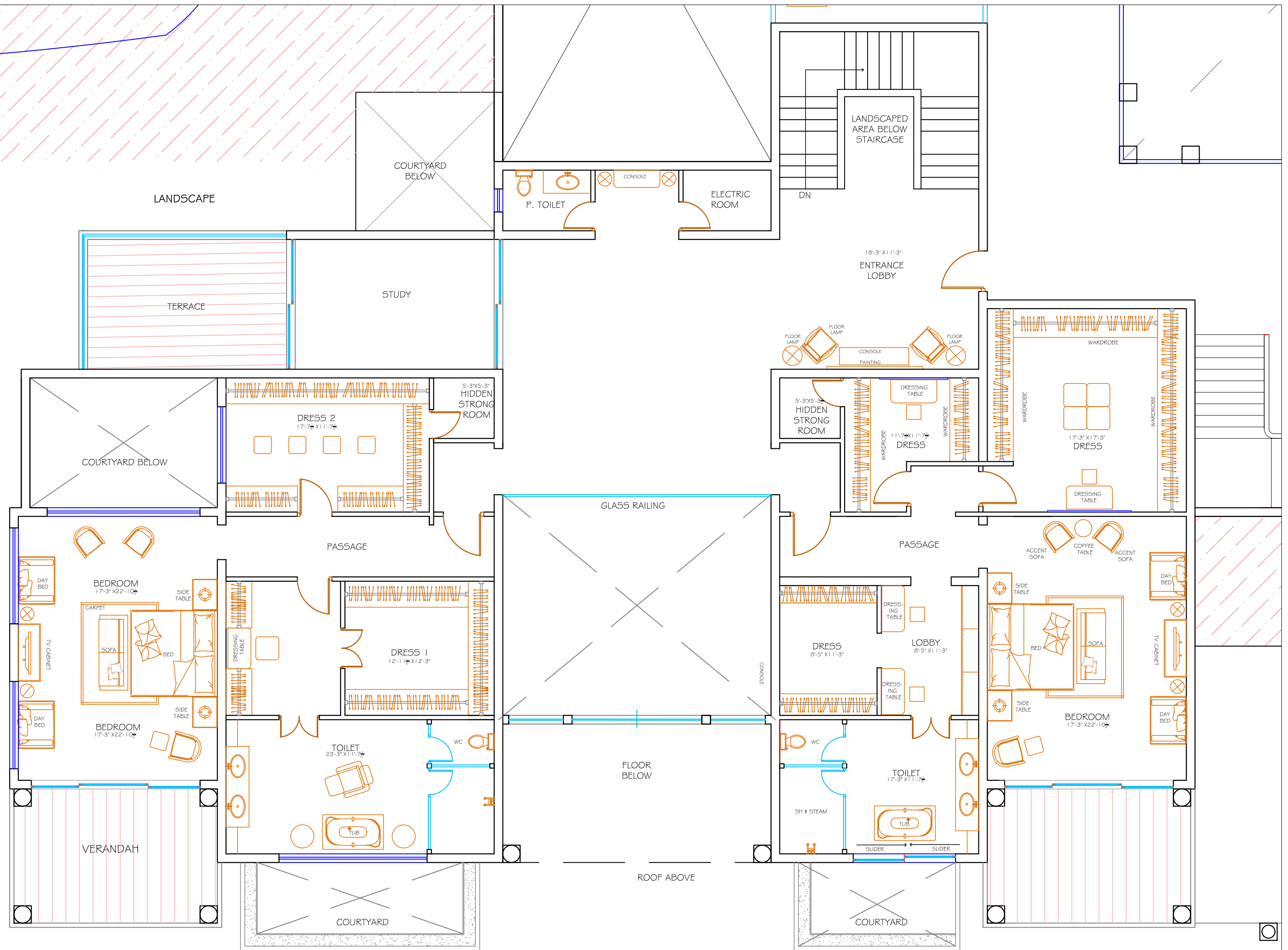
FIRST FLOOR
