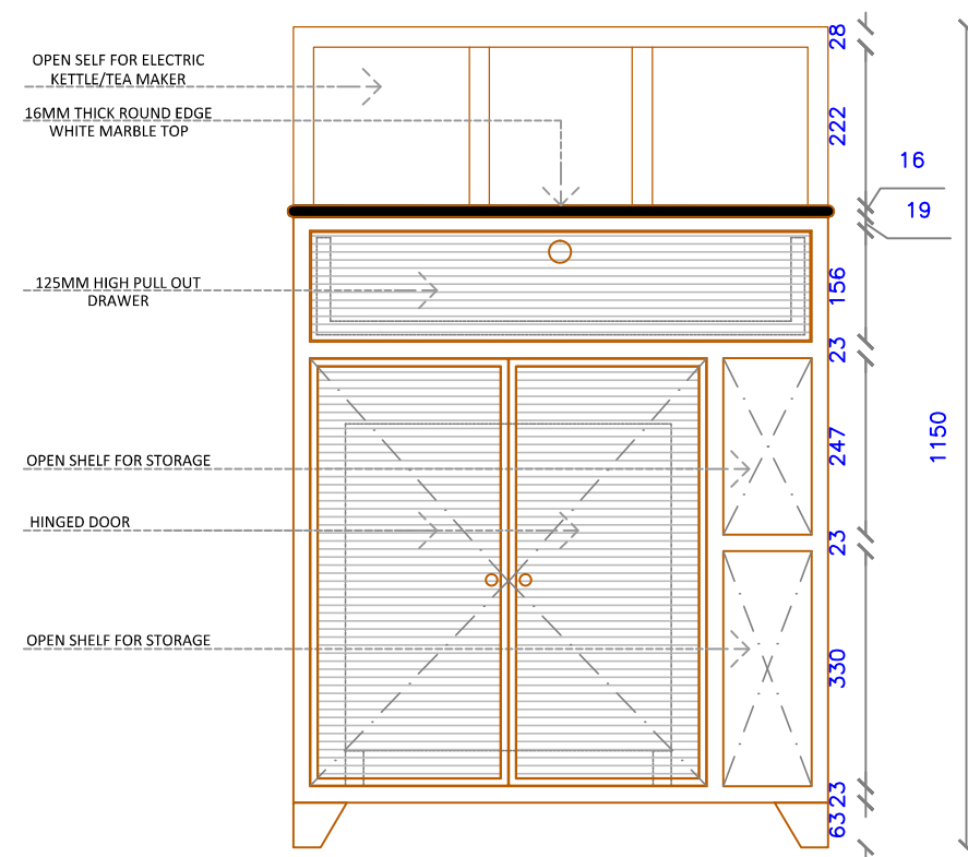
FRONT ELEVATION :MINI BAR
