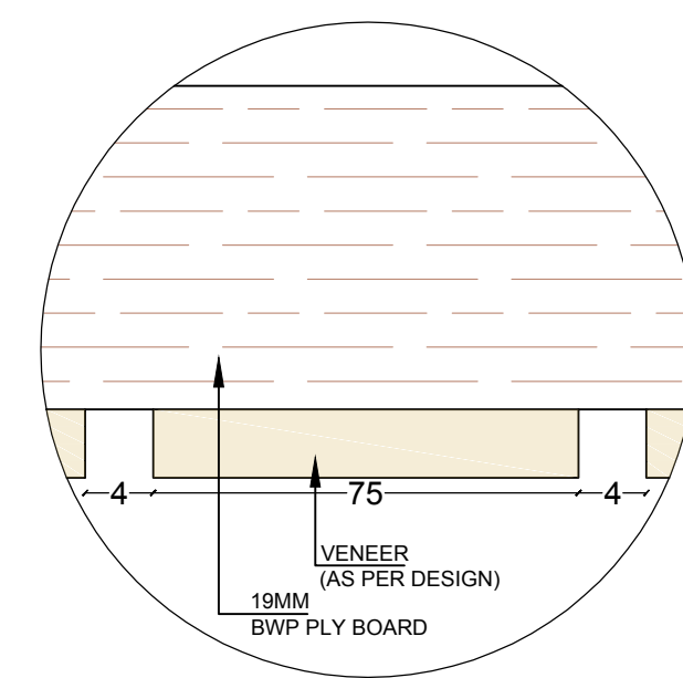
DETAIL AT X (SECTION)
