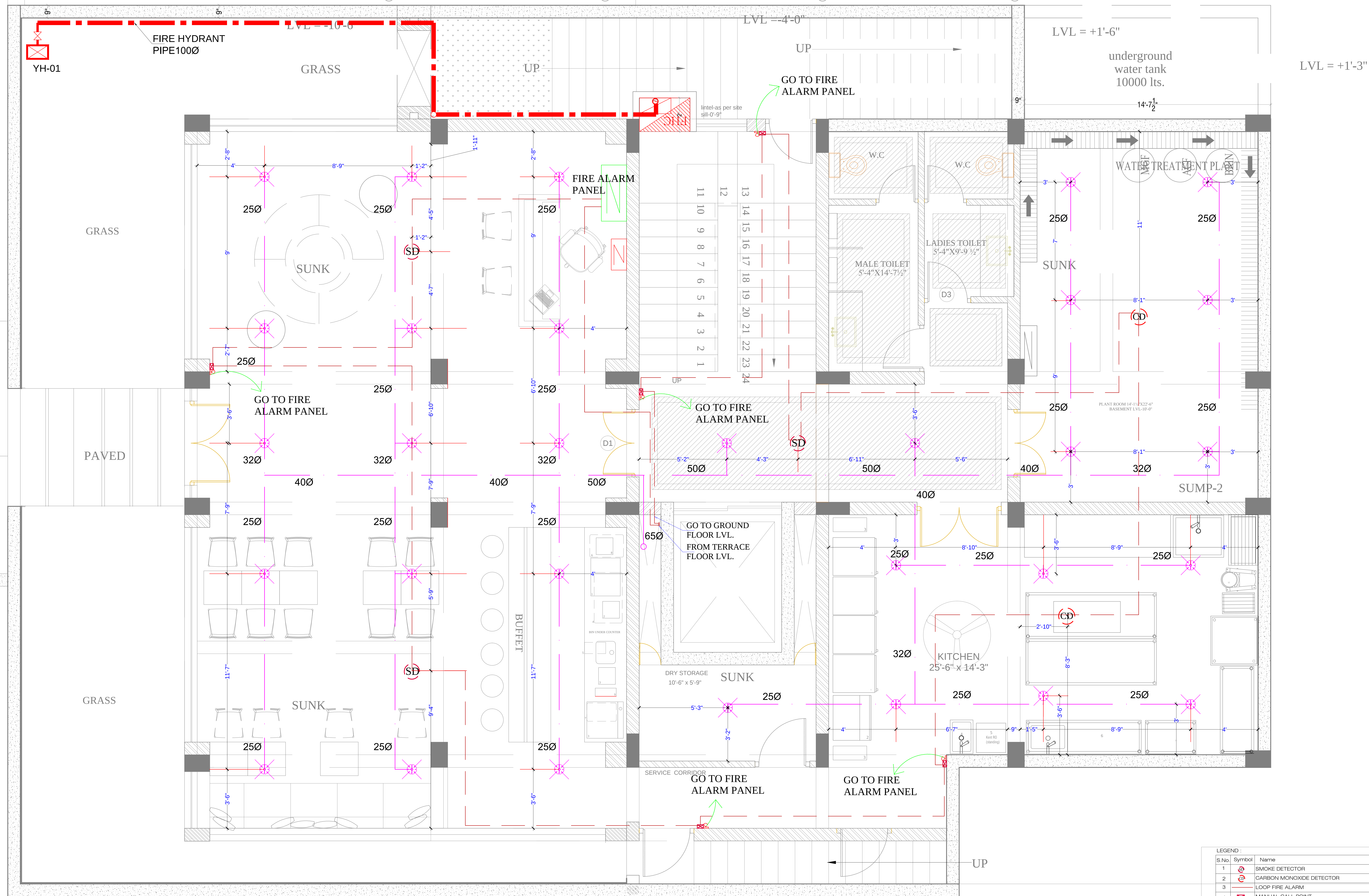
BASEMENT FLOOR
