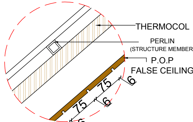
SECTION AT A
