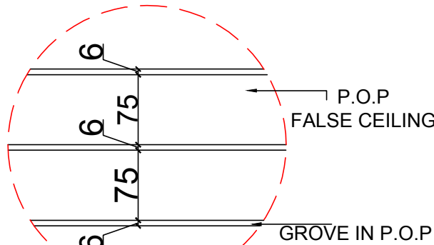
DETAIL AT A
