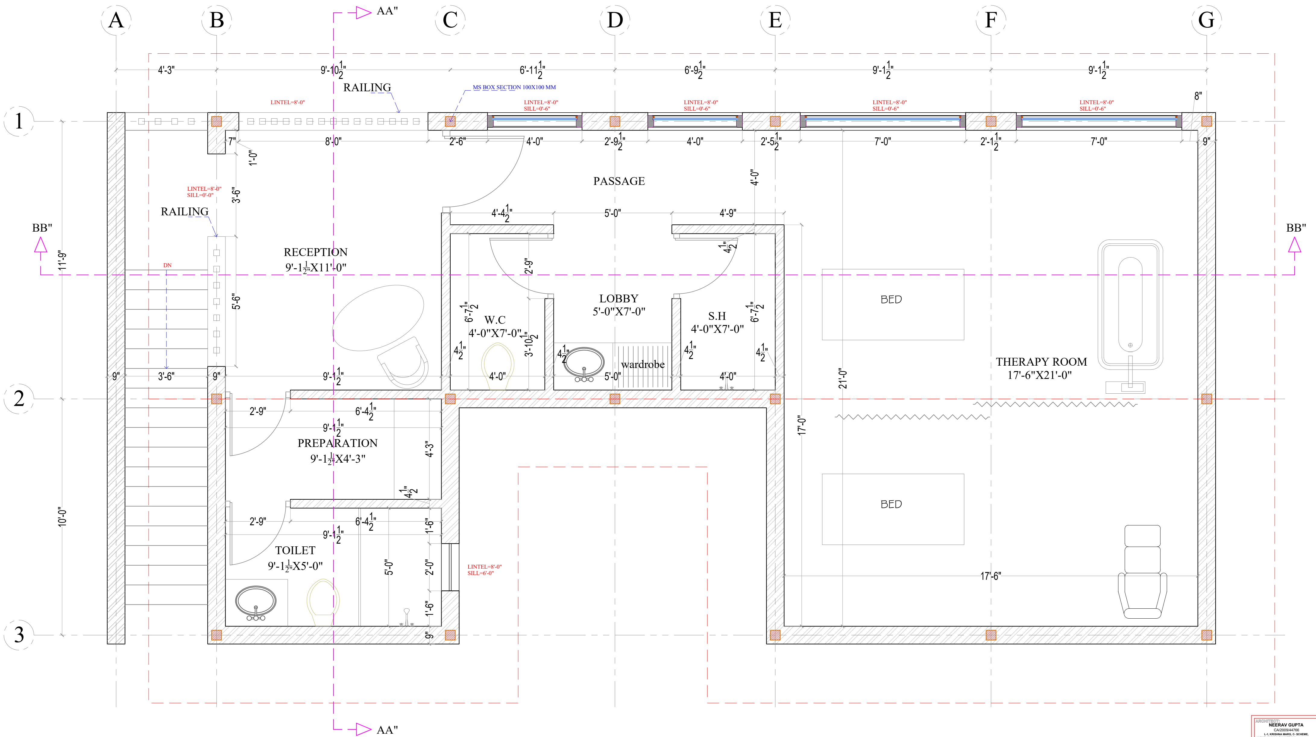
S.P.A WORKING DETAIL
