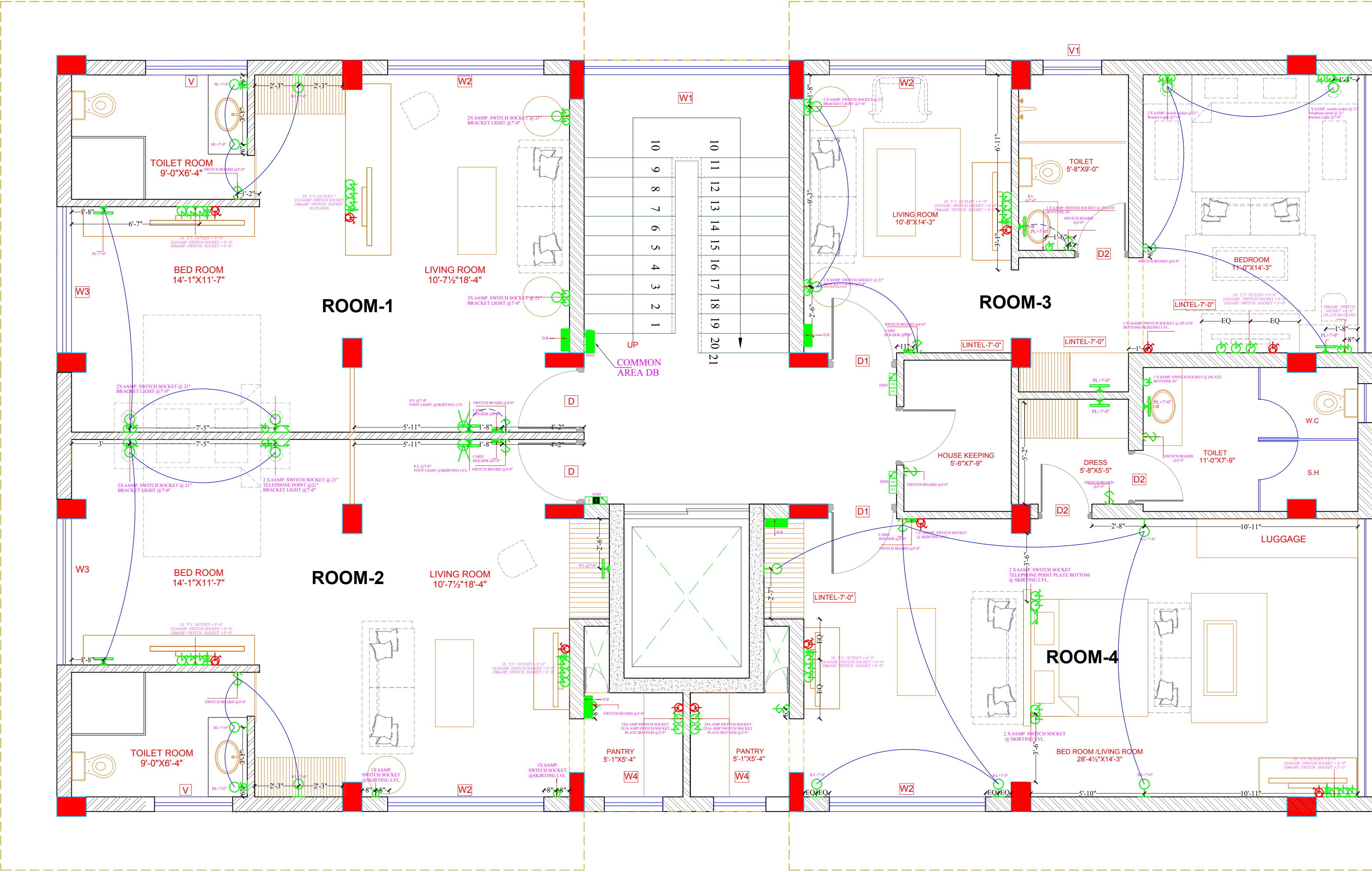
GROUND FLOOR WALL ELECTRICAL PLAN
