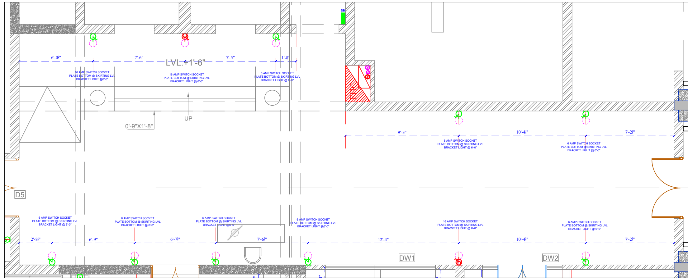
LOBBY WALL ELECTRICAL
