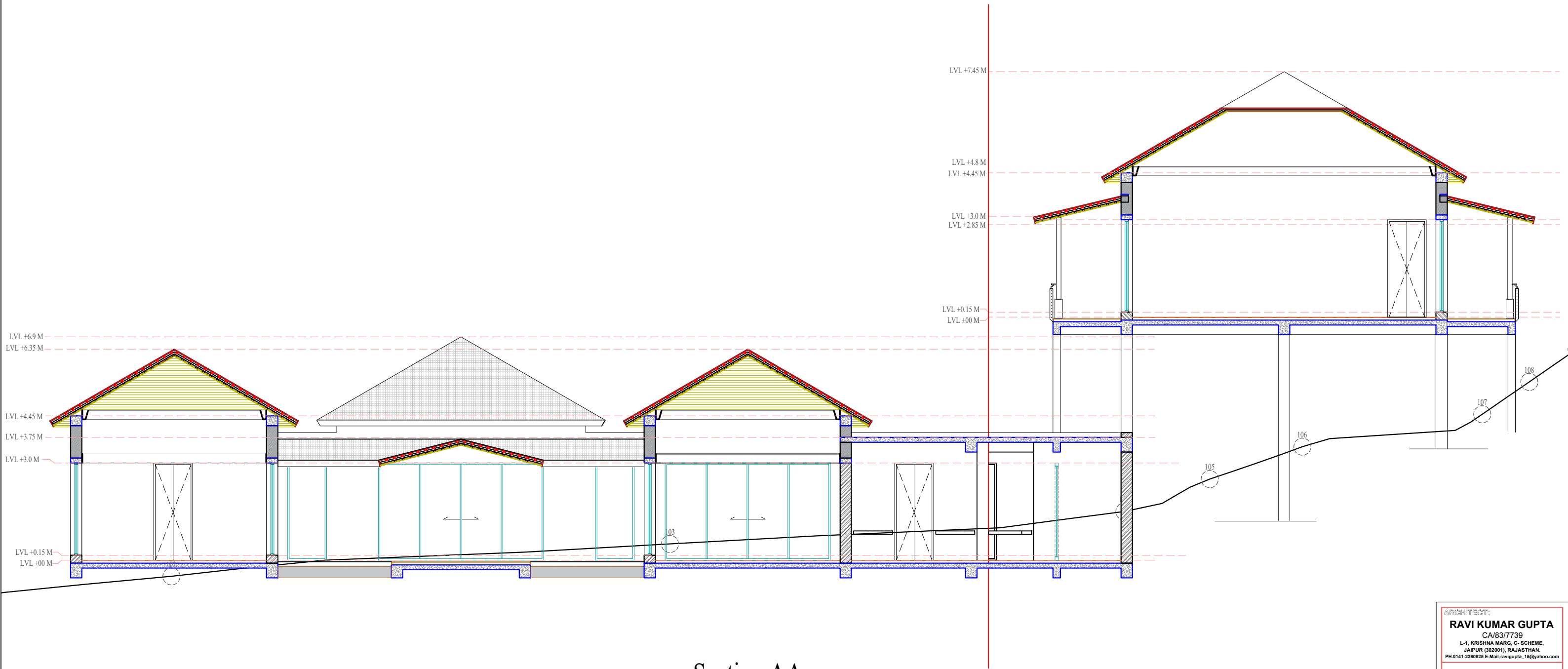
Section AA
