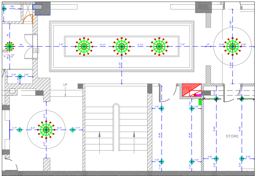
REFLECTED CEILING ELECTRICAL
