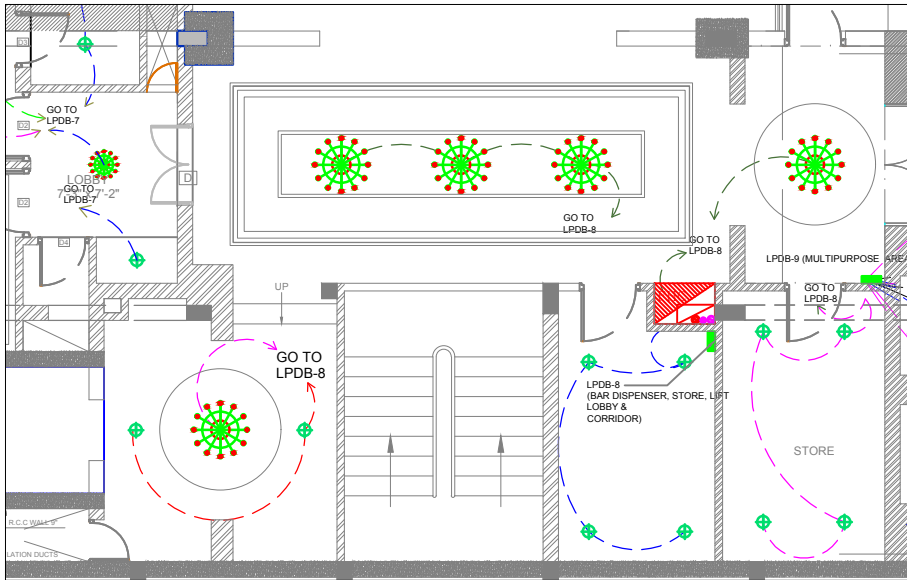
REFLECTED CEILING WIRE DIAGRAM
