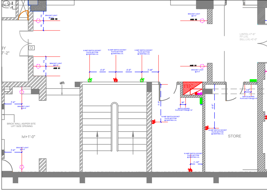
WALL ELECTRICAL
