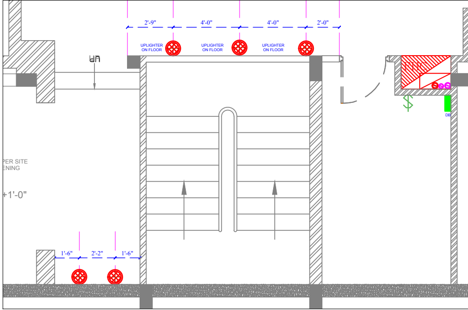
FLOOR ELECTRICAL
