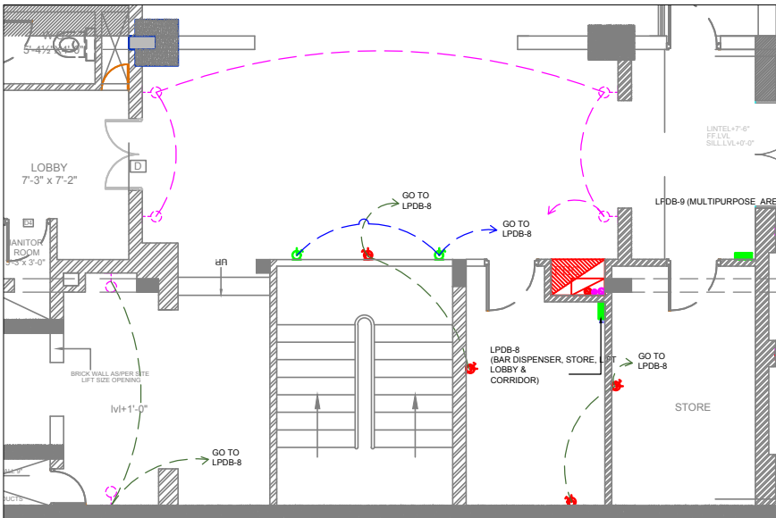
WALL WIRE DIAGRAM
