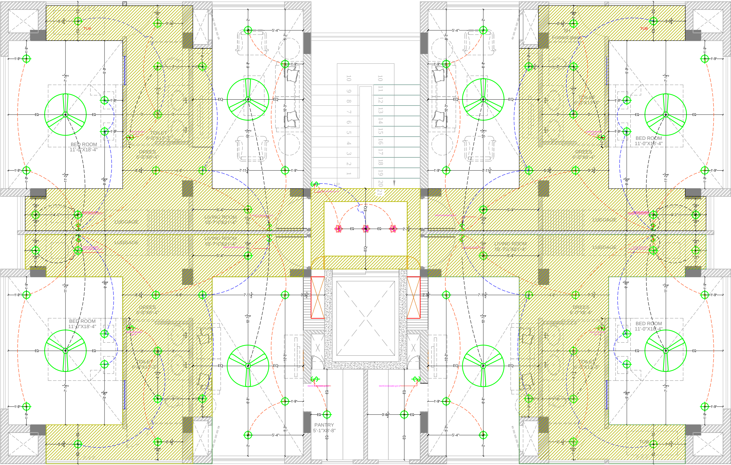
TYPICAL FLOOR CEILING ELECTRICAL PLAN
