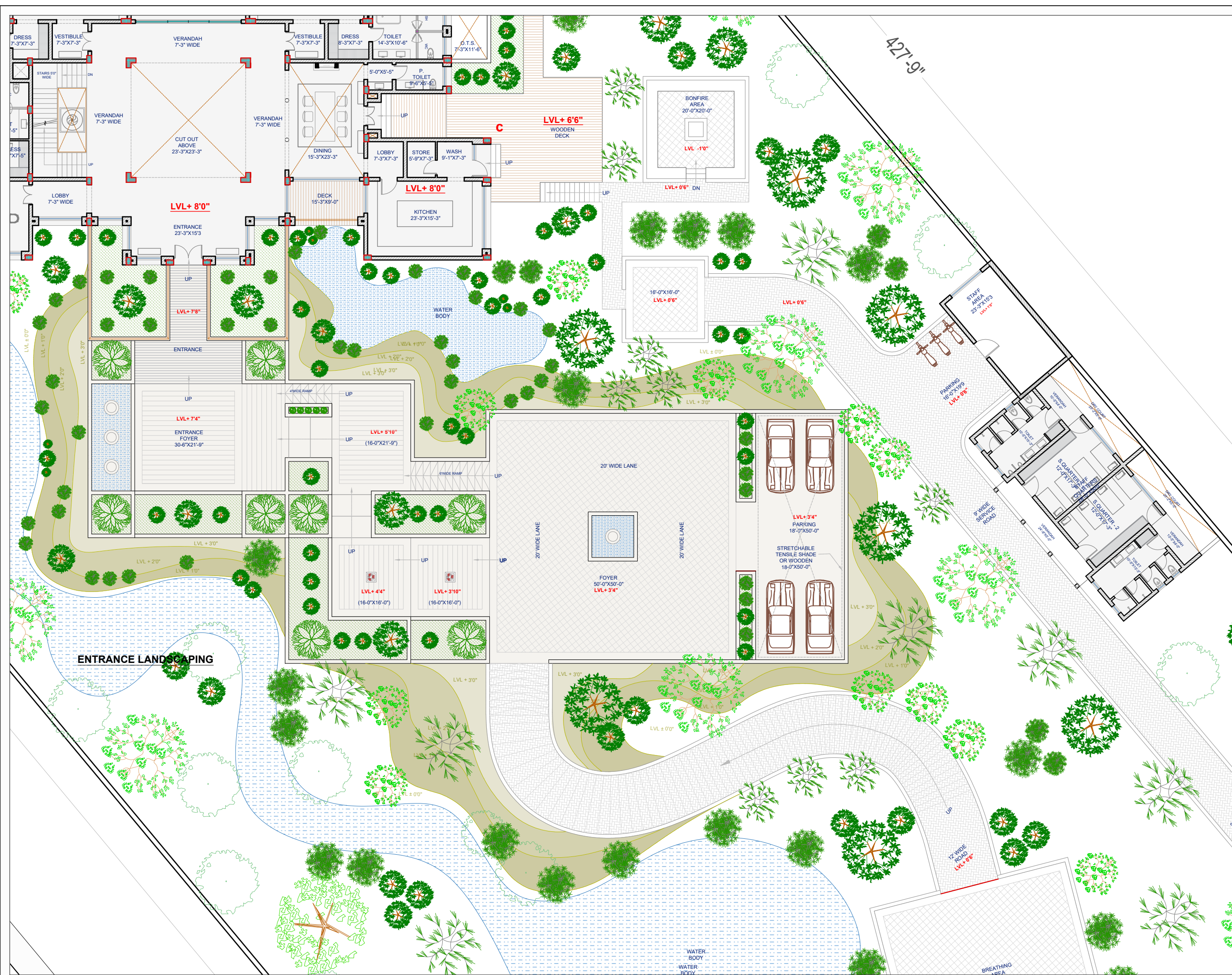
KEY PLAN
