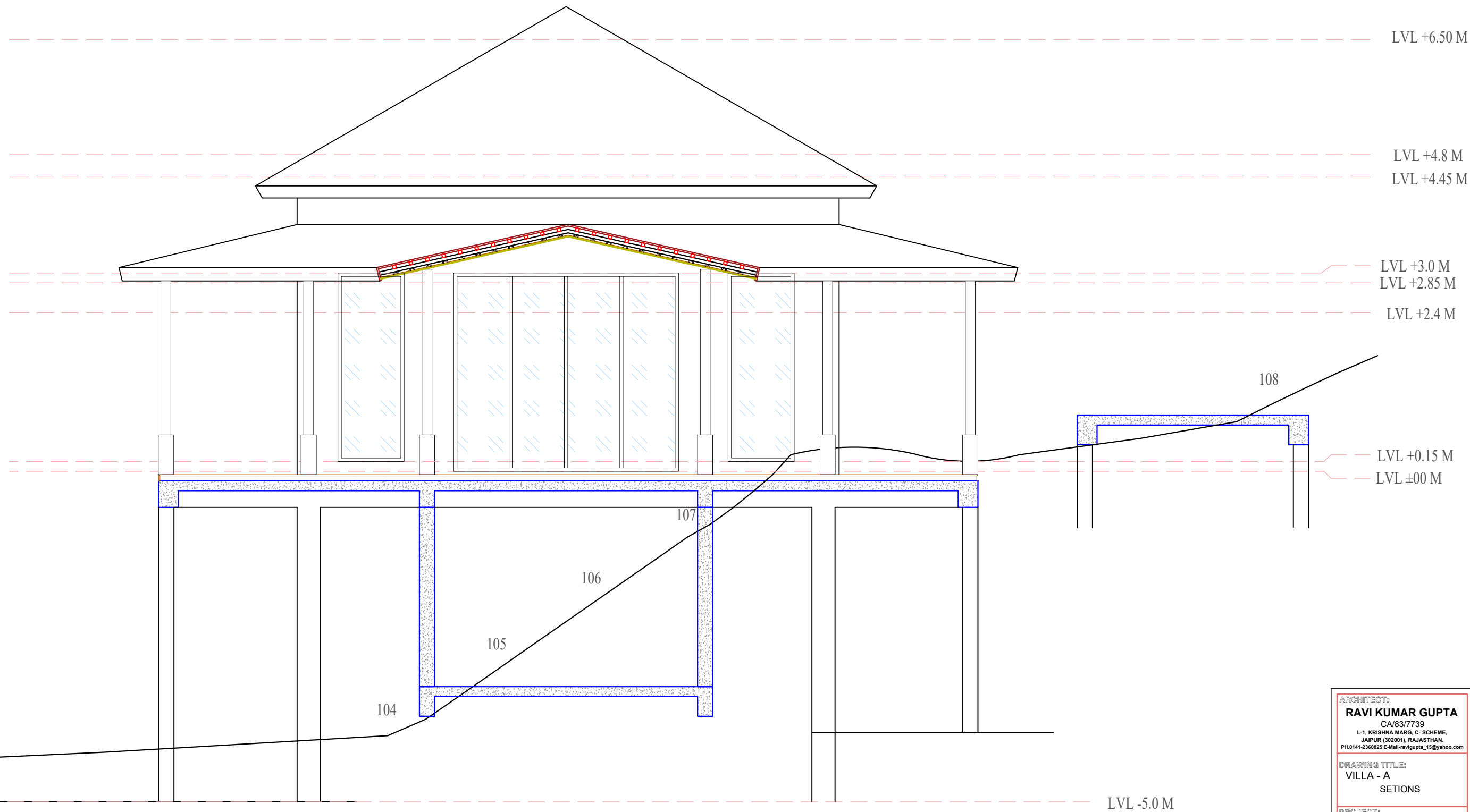
Section CC (Sitting area)
