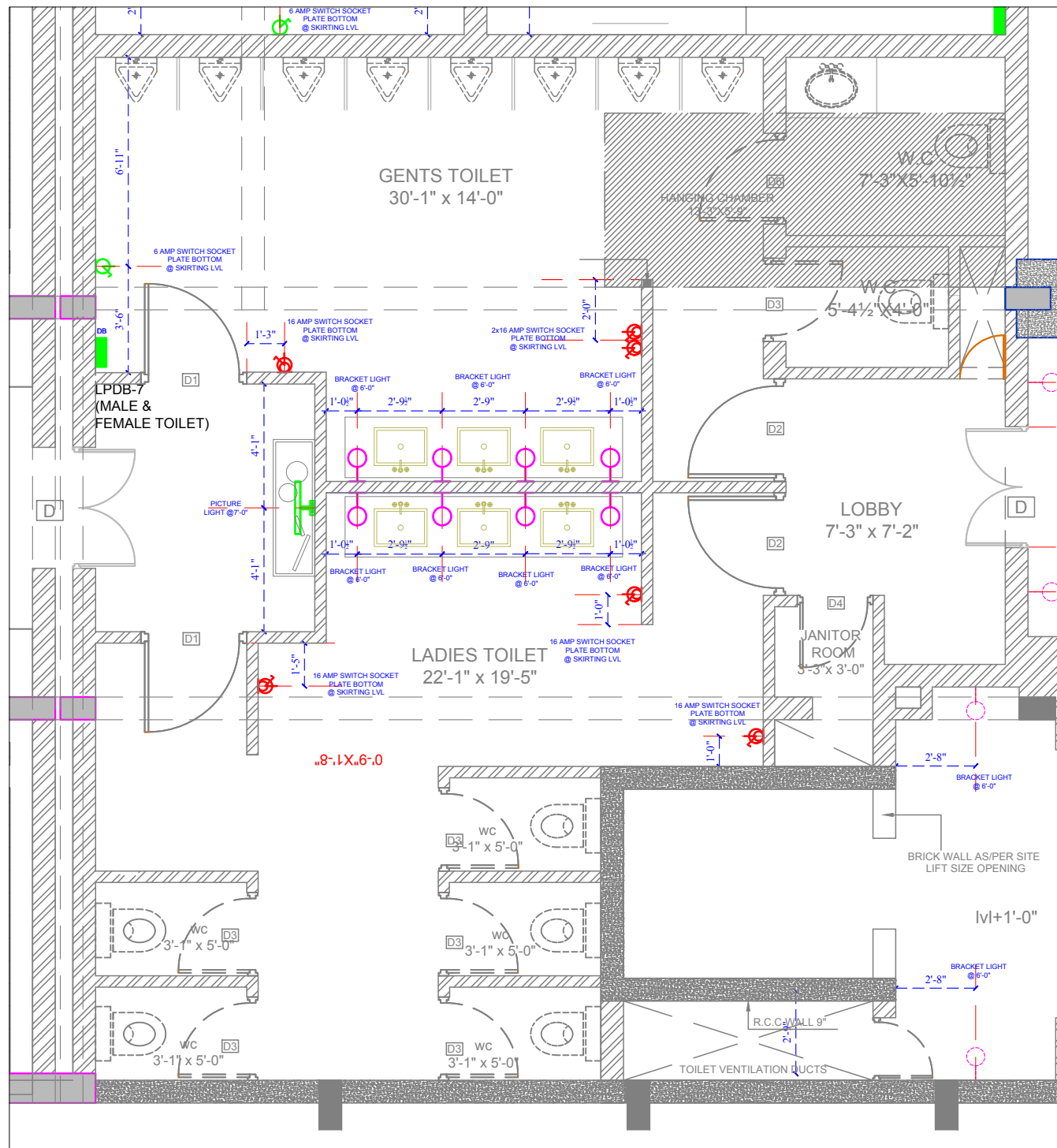
TOILET WALL ELECTRICAL PLAN
