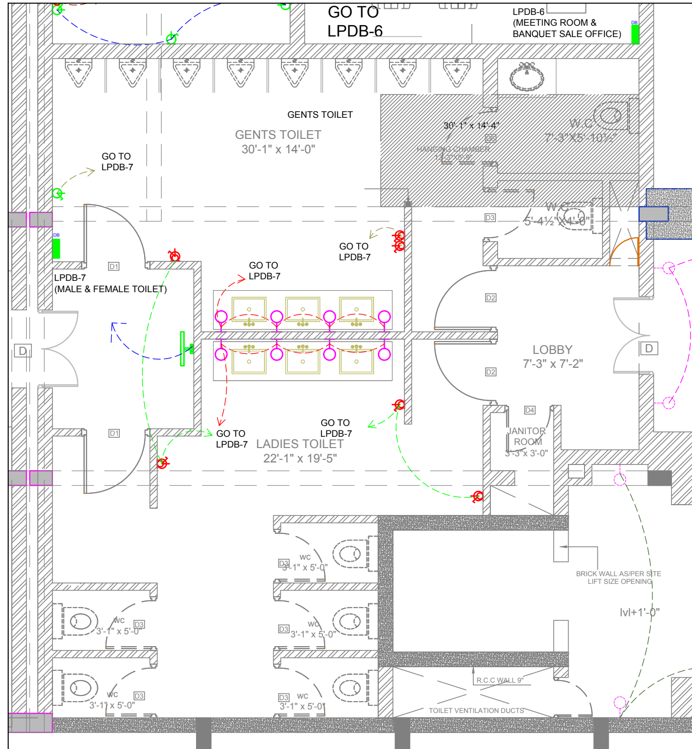
TOILET WALL WIRE DIAGRAM
