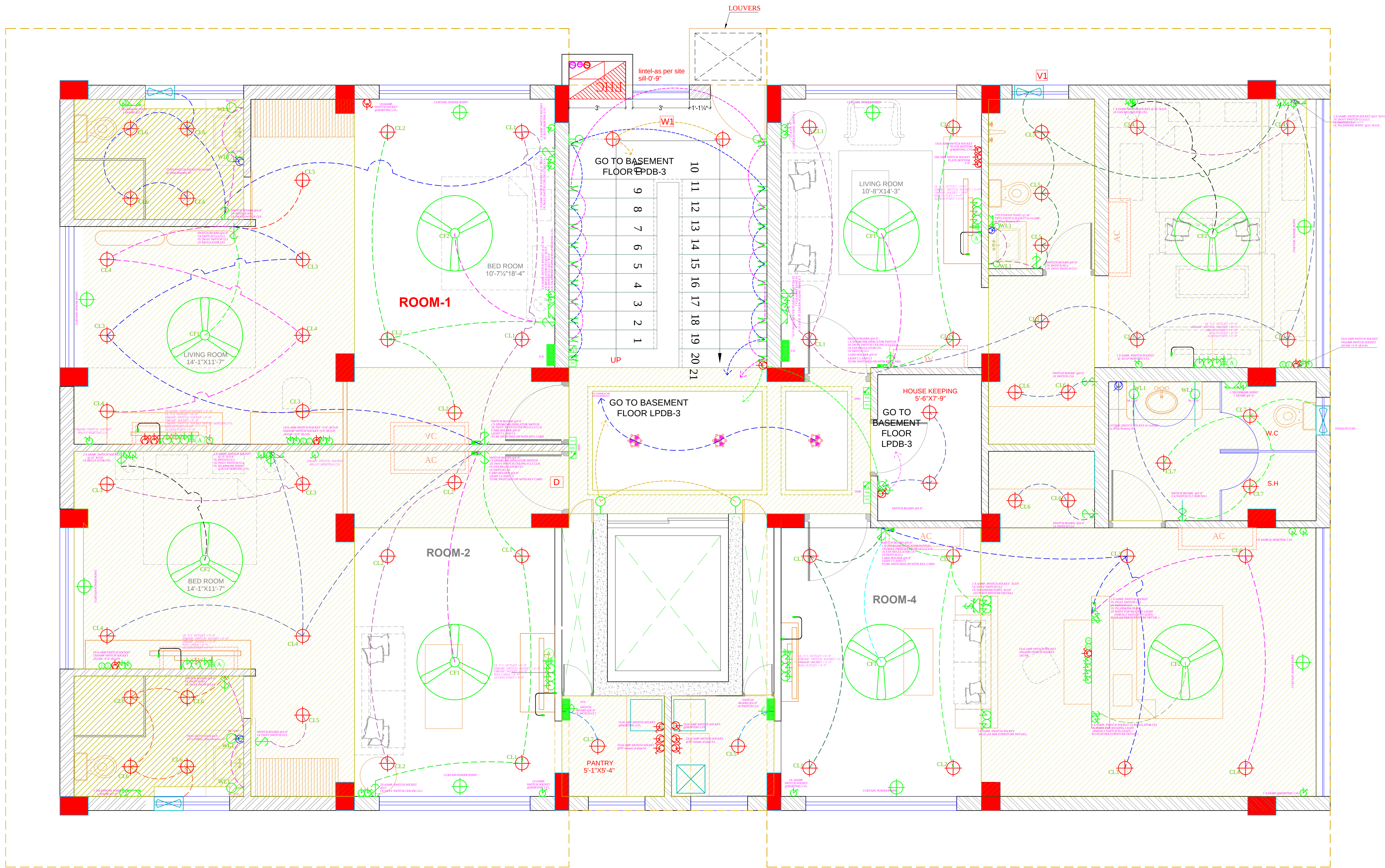
GROUND FLOOR WIRING DIAGRAM
