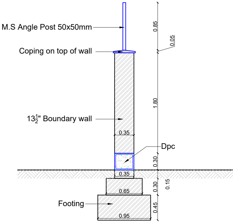
TYPICAL BOUNDARY WALL SECTION
