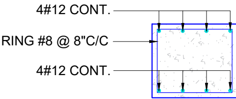
DPC DETAIL
