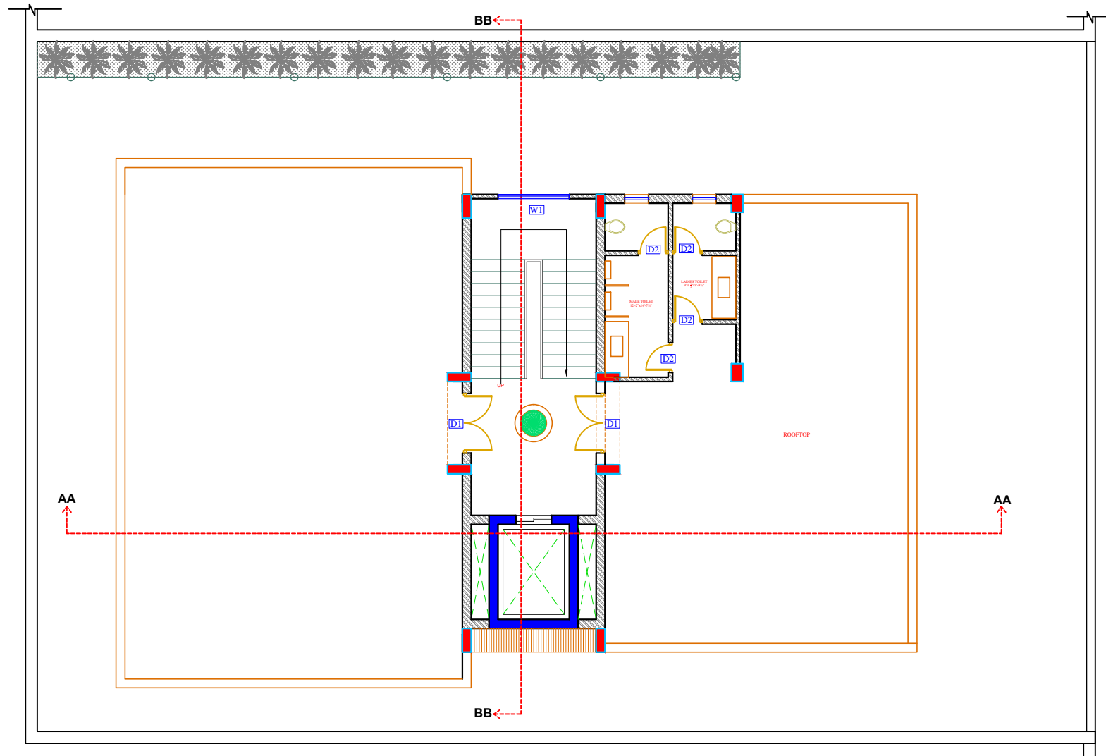
TERRACE FLOOR
