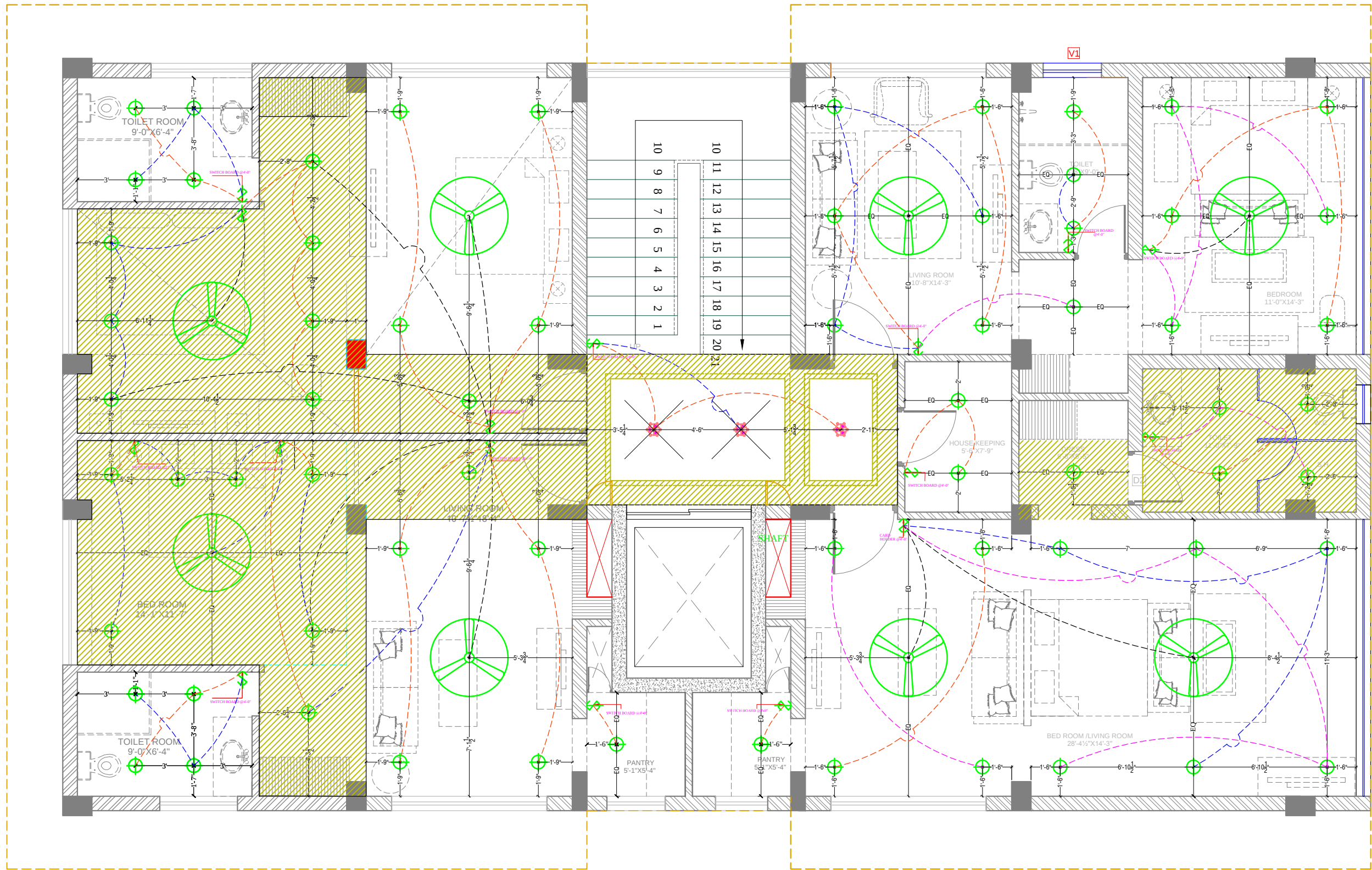
GROUND FLOOR CEILING ELECTRICAL PLAN
