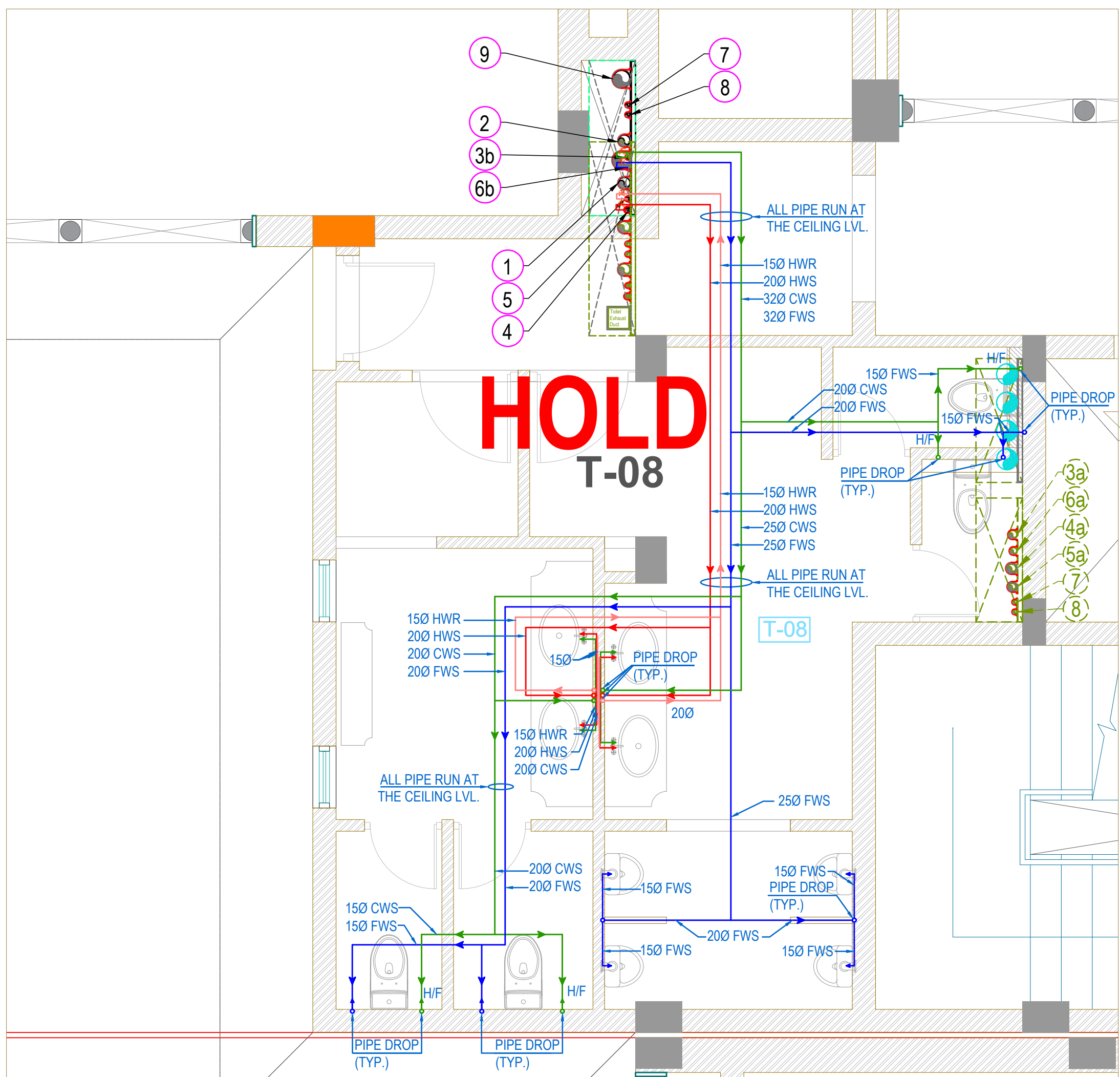
TOILET-08 FOR GROUND FLOOR (WATER SUPPLY LAYOUT)
