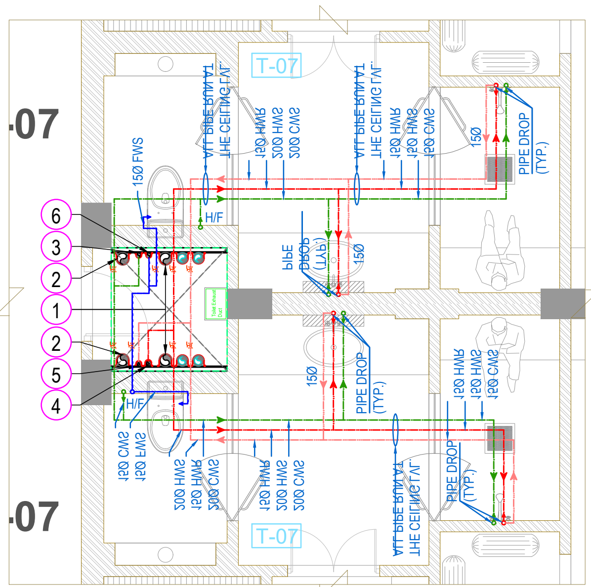
TOILET-07 FOR GROUND FLOOR (WATER SUPPLY LAYOUT)
