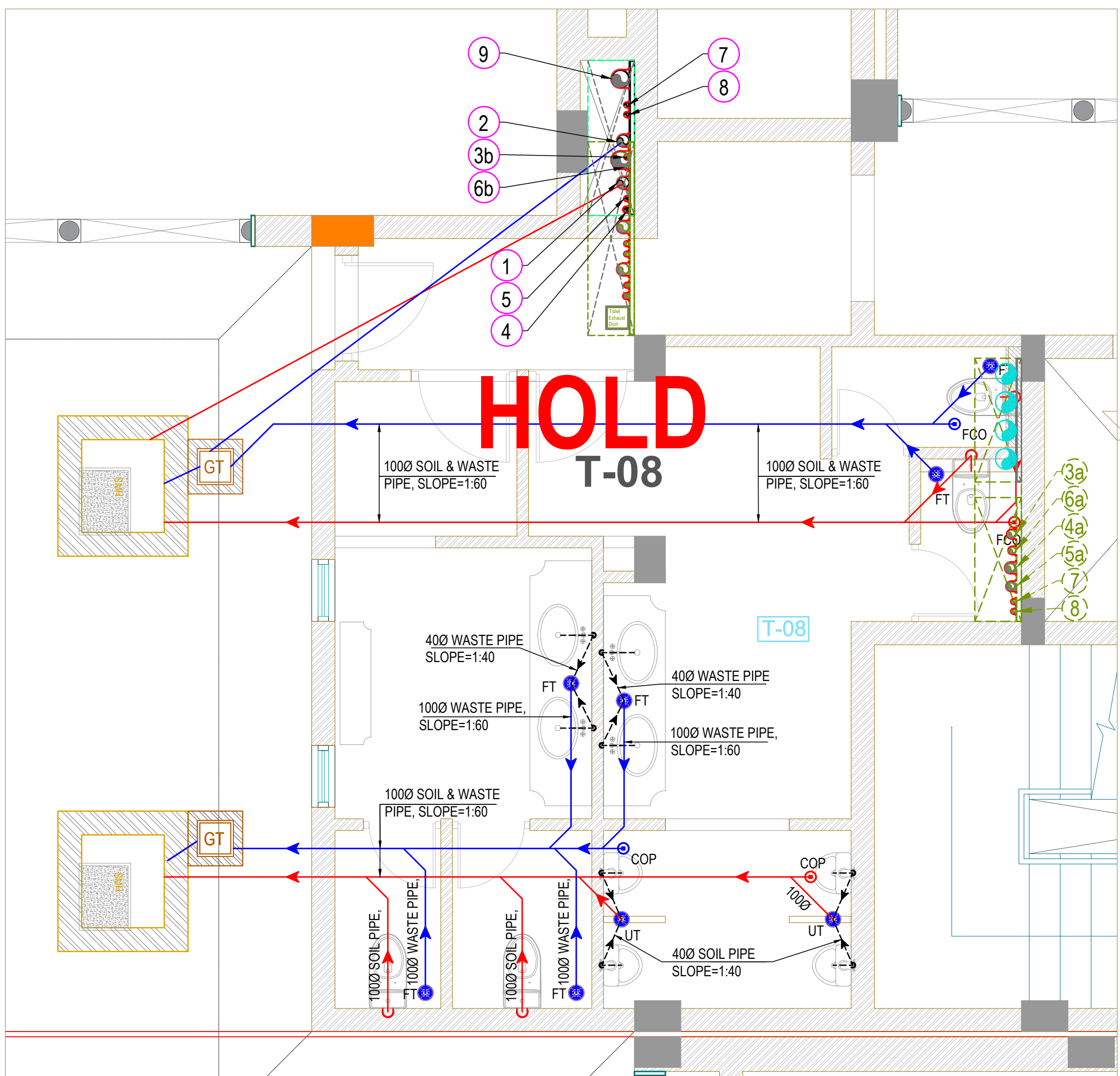
TOILET-08 FOR GROUND FLOOR (DRAINAGE LAYOUT)
