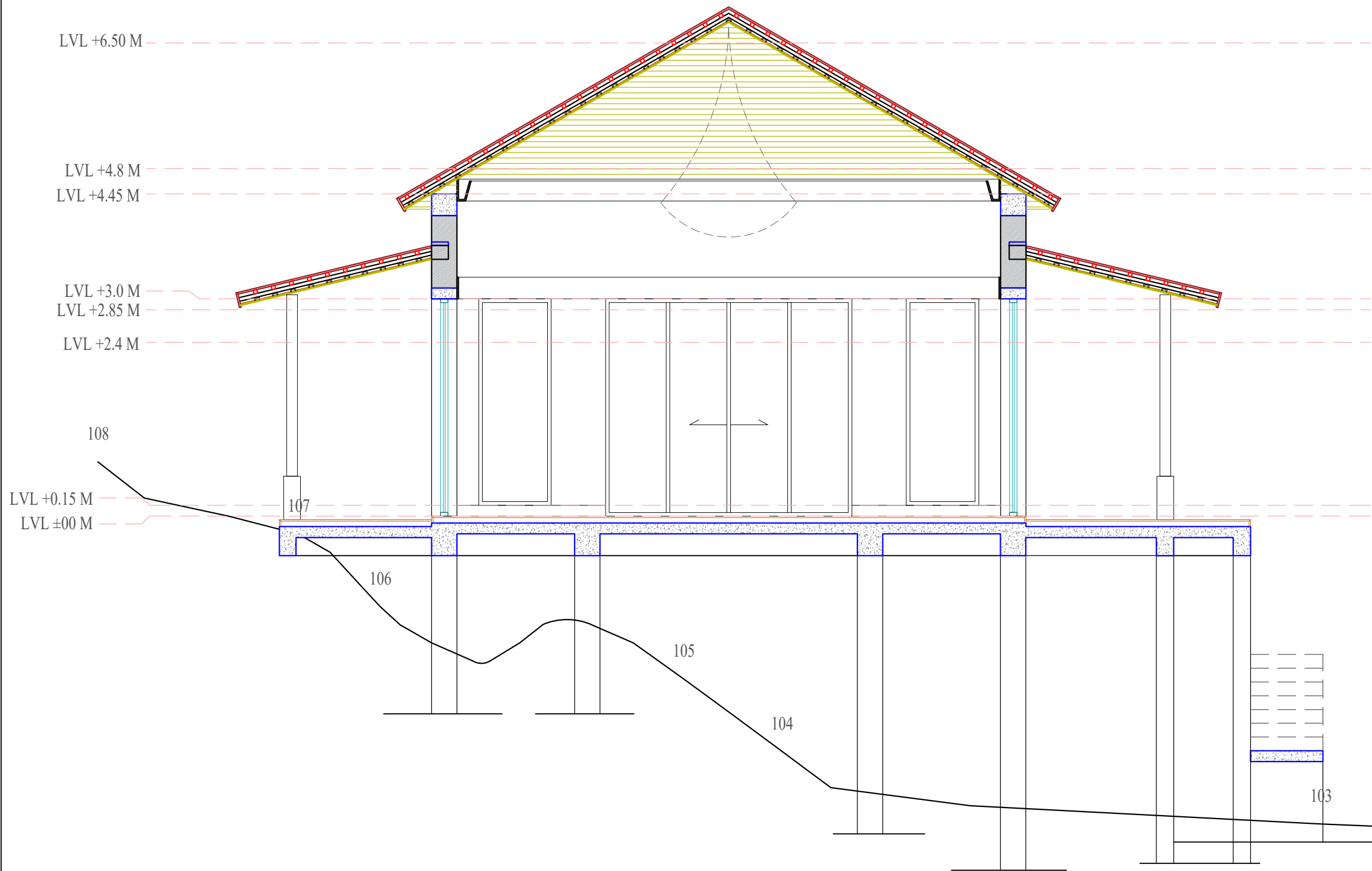
Section DD(Living room)
